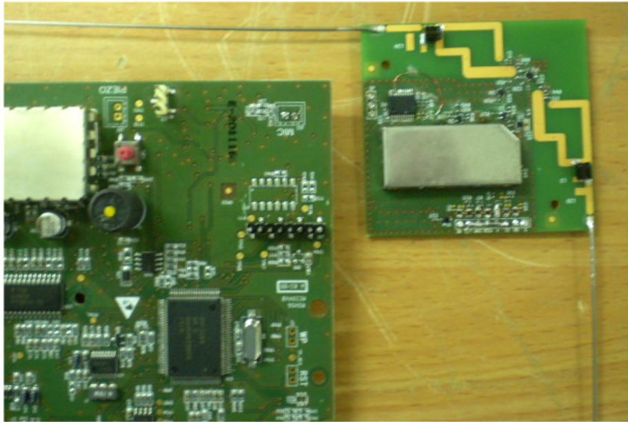
Photograph No.11 RF 315 MHz module removed from the main PCB
