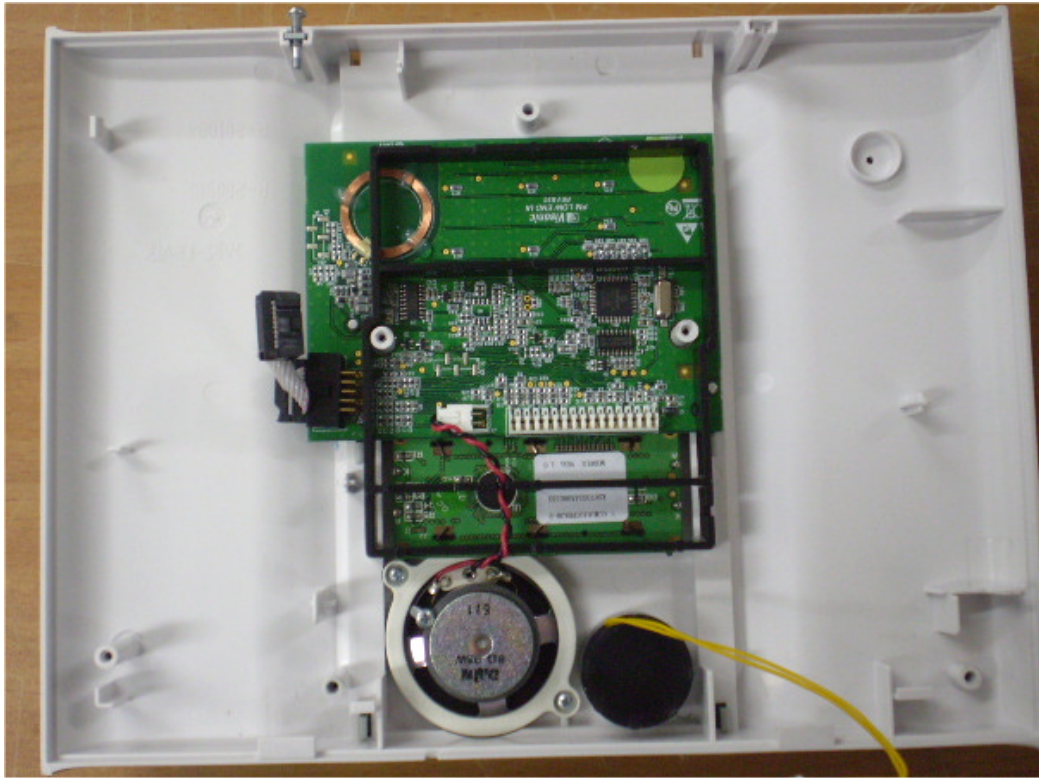
Photograph No.15 Proximity module in the EUT case
