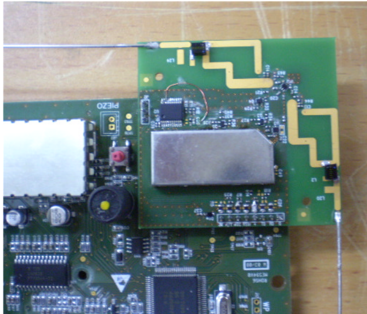
Photograph No.10 Close view of RF 315 MHz module on the main PCB
