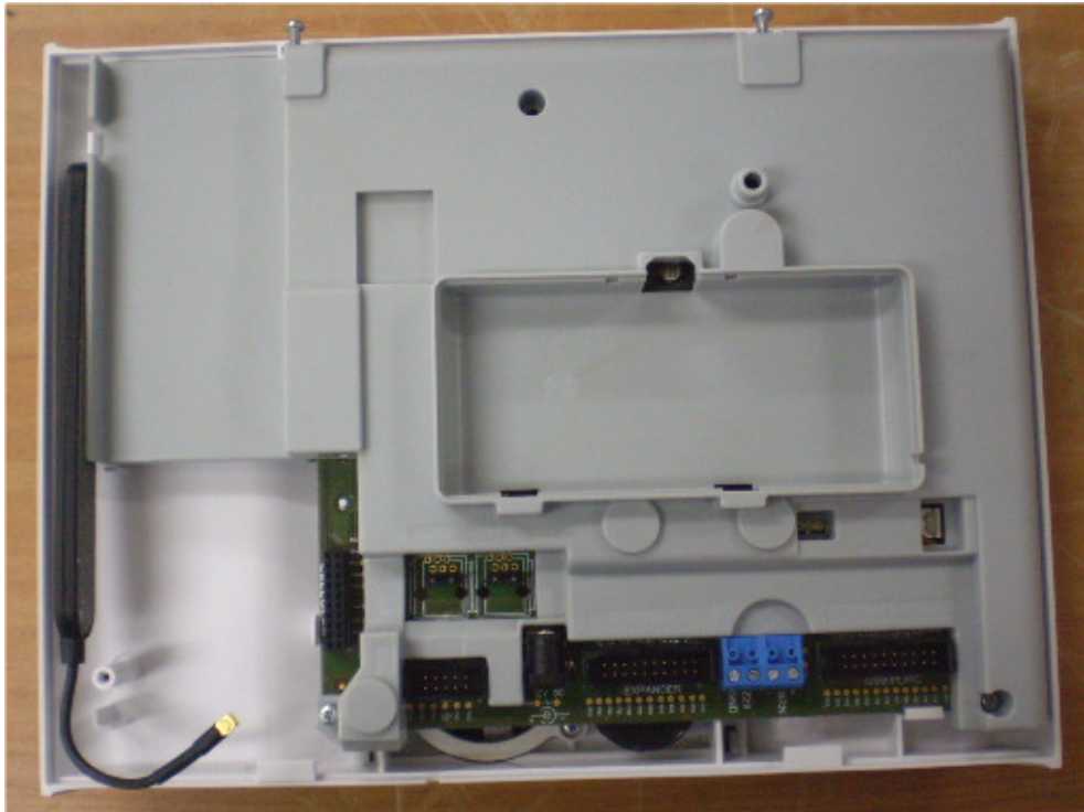
Photograph No.4 PowerMaxComplete with battery pack removed
