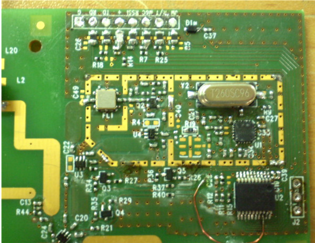
Photograph No.13 RF 315 MHz module without shield
