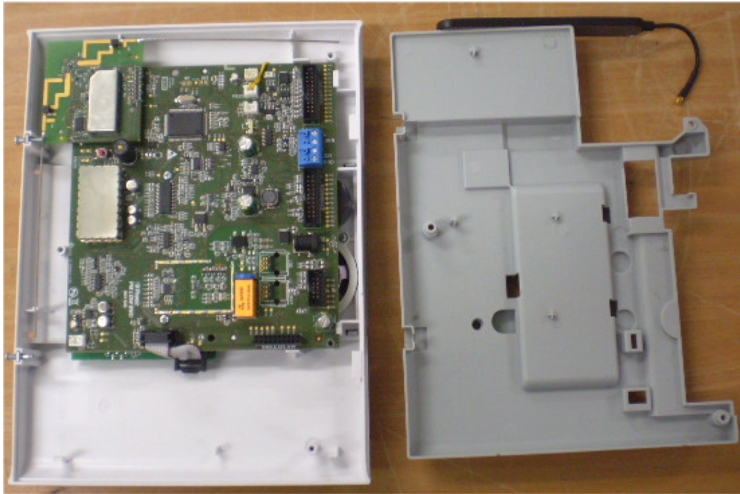
Photograph No.5 PowerMaxComplete internal view with cover removed
