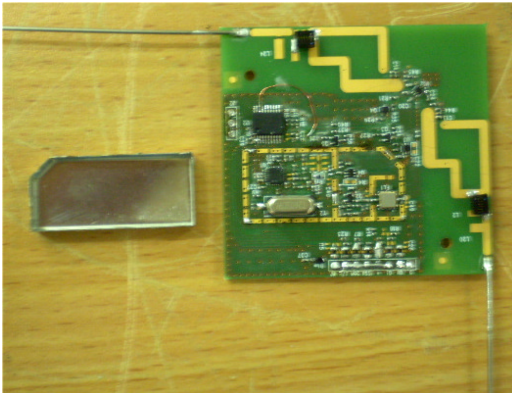
Photograph No.12 RF 315 MHz module with shield removed
