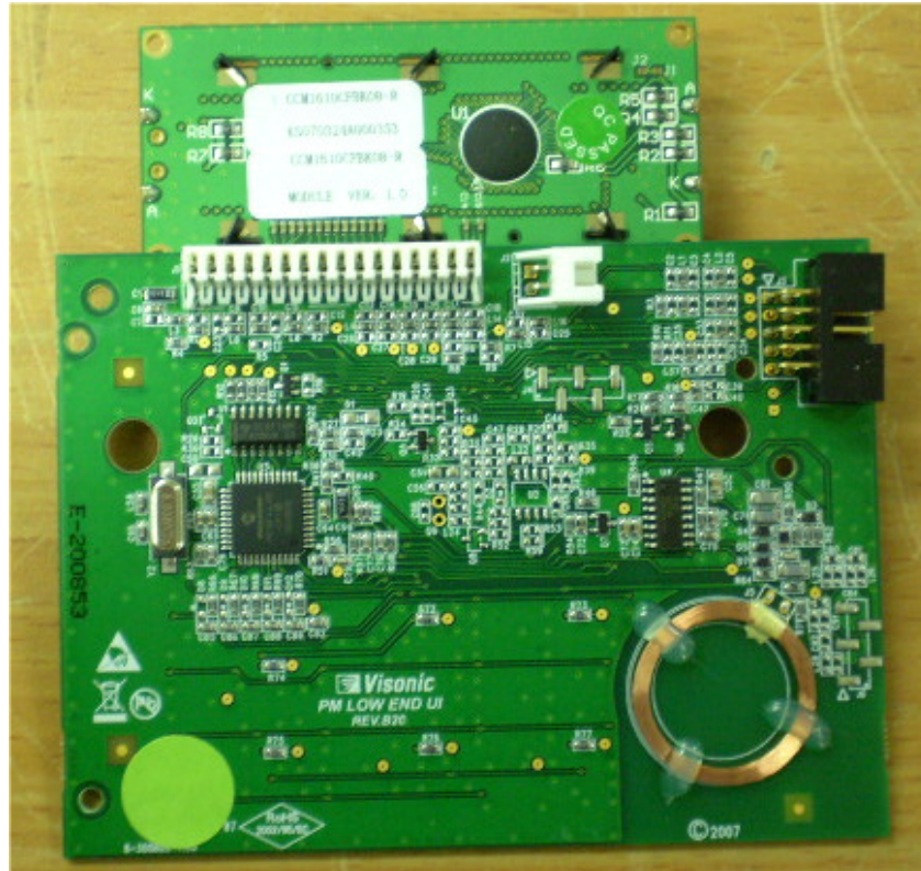
Photograph No.17 Proximity module PCB front view
