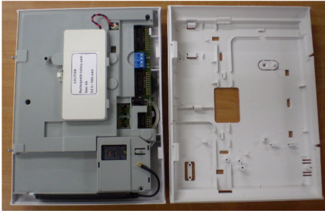
Photograph No.1 PowerMaxComplete internal view
