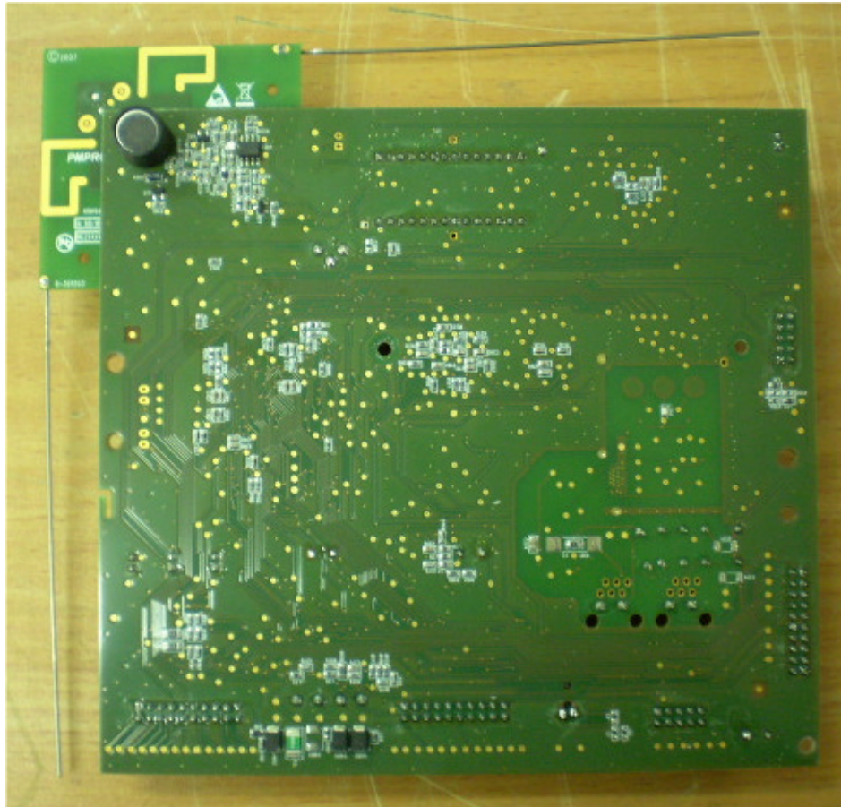
Photograph No.8 PowerMaxComplete main PCB second side view
