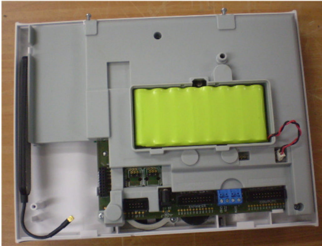
Photograph No.3 PowerMaxComplete internal view with battery pack open
