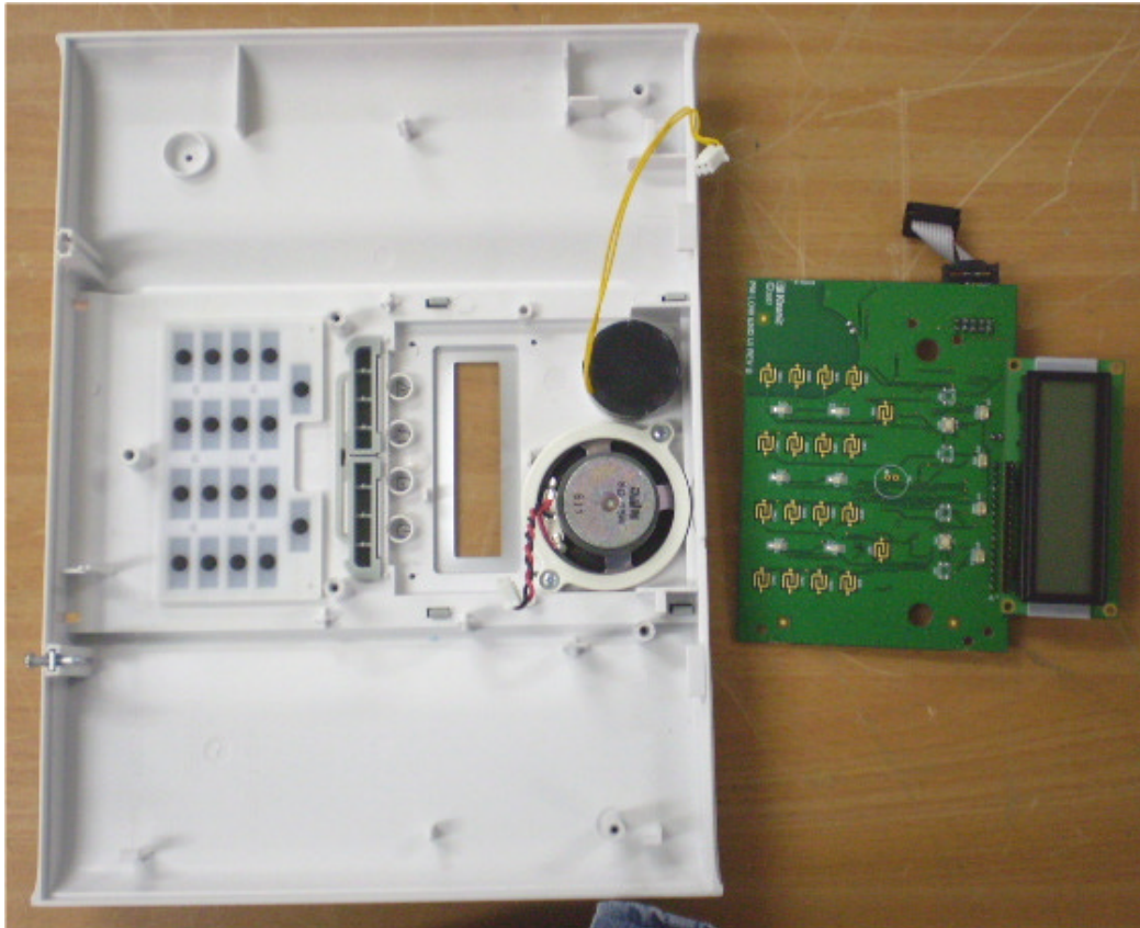
Photograph No.16 Proximity module removed from the EUT case
