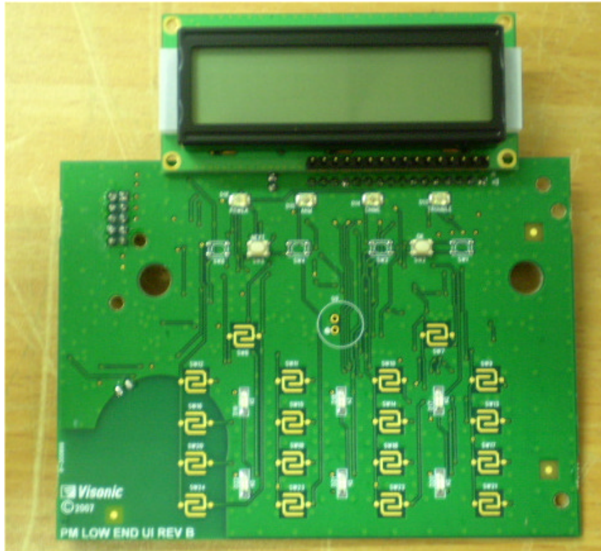
Photograph No.18 Proximity module PCB second side view
